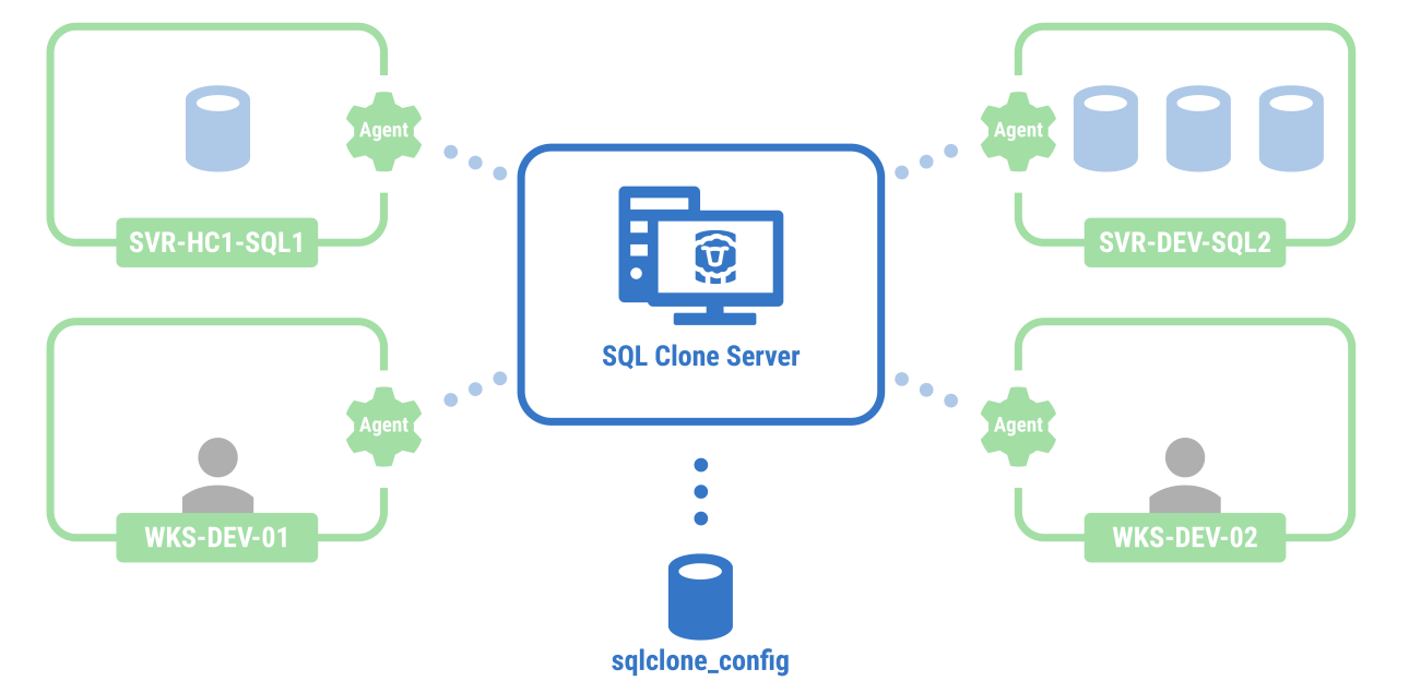
SQL Clone Sample Architecture
